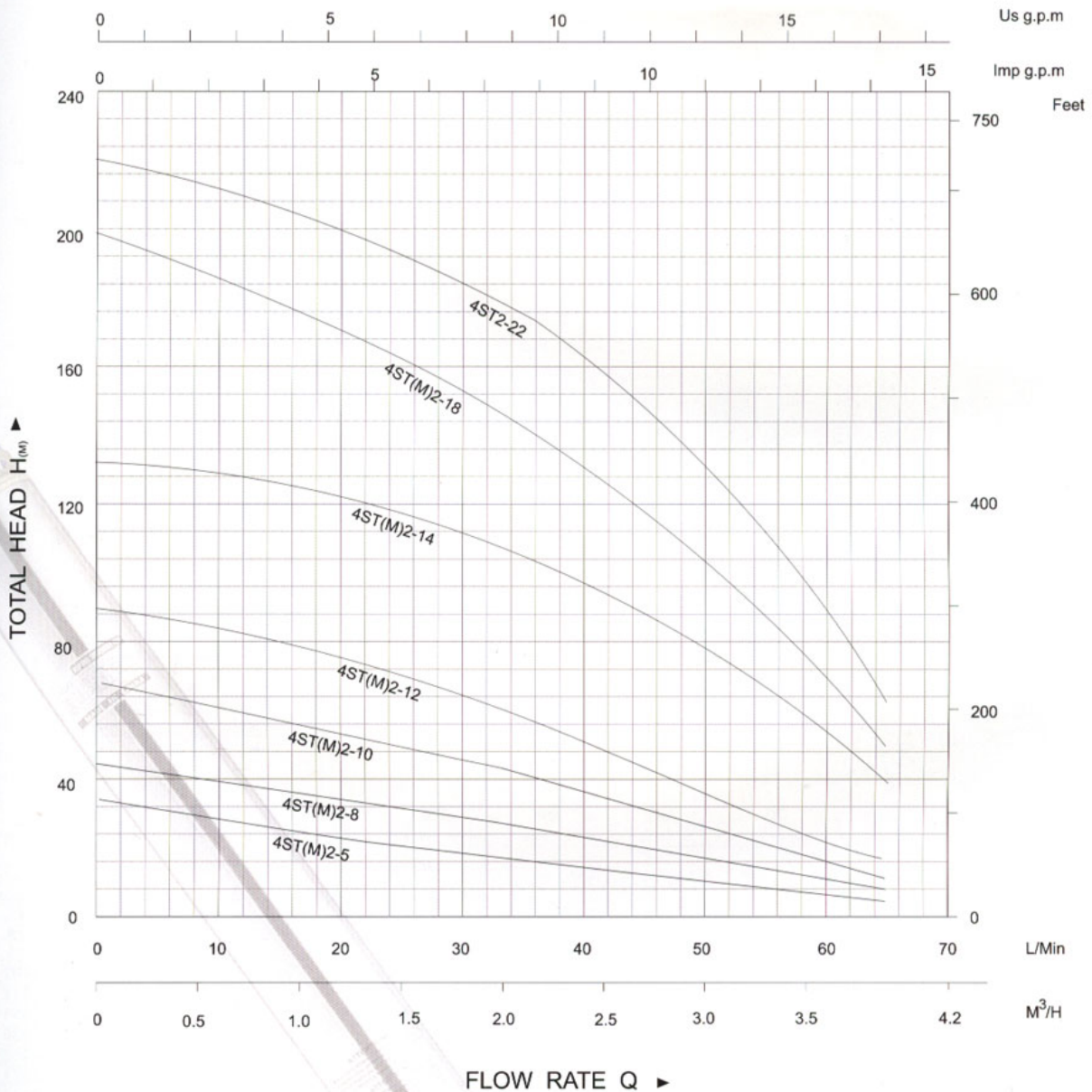
PERFORMANCE CHART AT n=2900rpm
