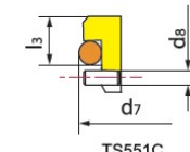
TS551C G9 (DIN24960)
