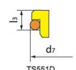
TS551D G6 (DIN24960)
