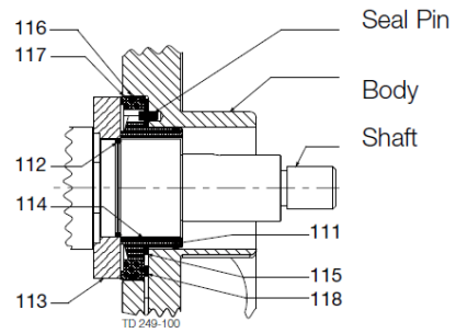
Double Mechanical Seal
