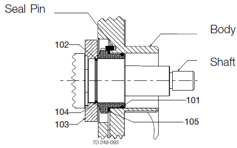
Single Mechanical Seal
