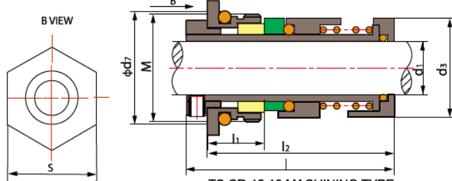
TS CR-12,16 MACHINING TYPE
