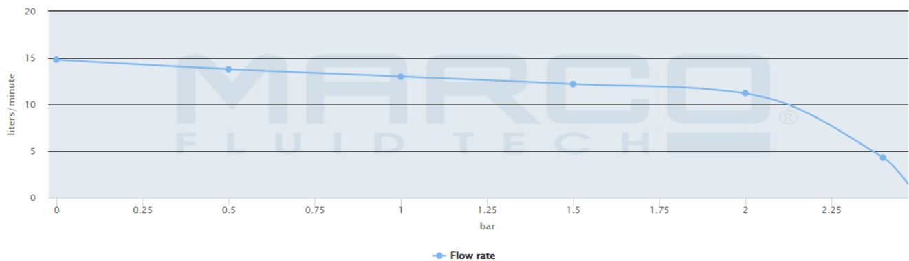
Flow rate
