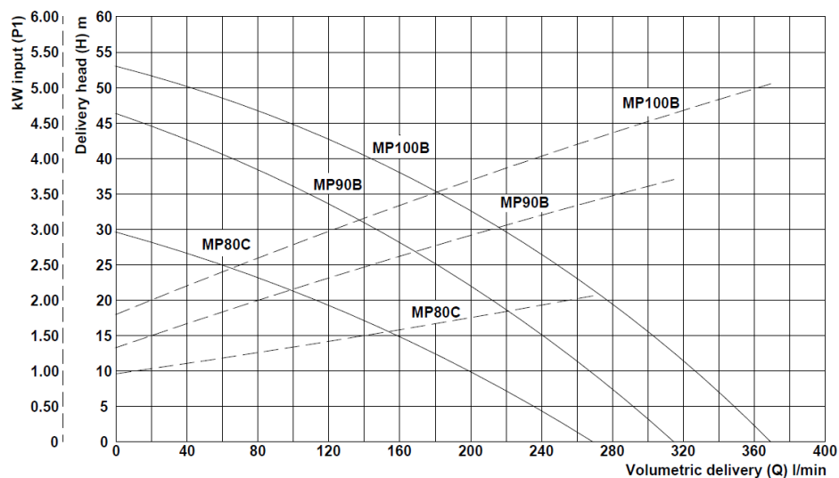
Hydraulic performance curves (open impeller)
