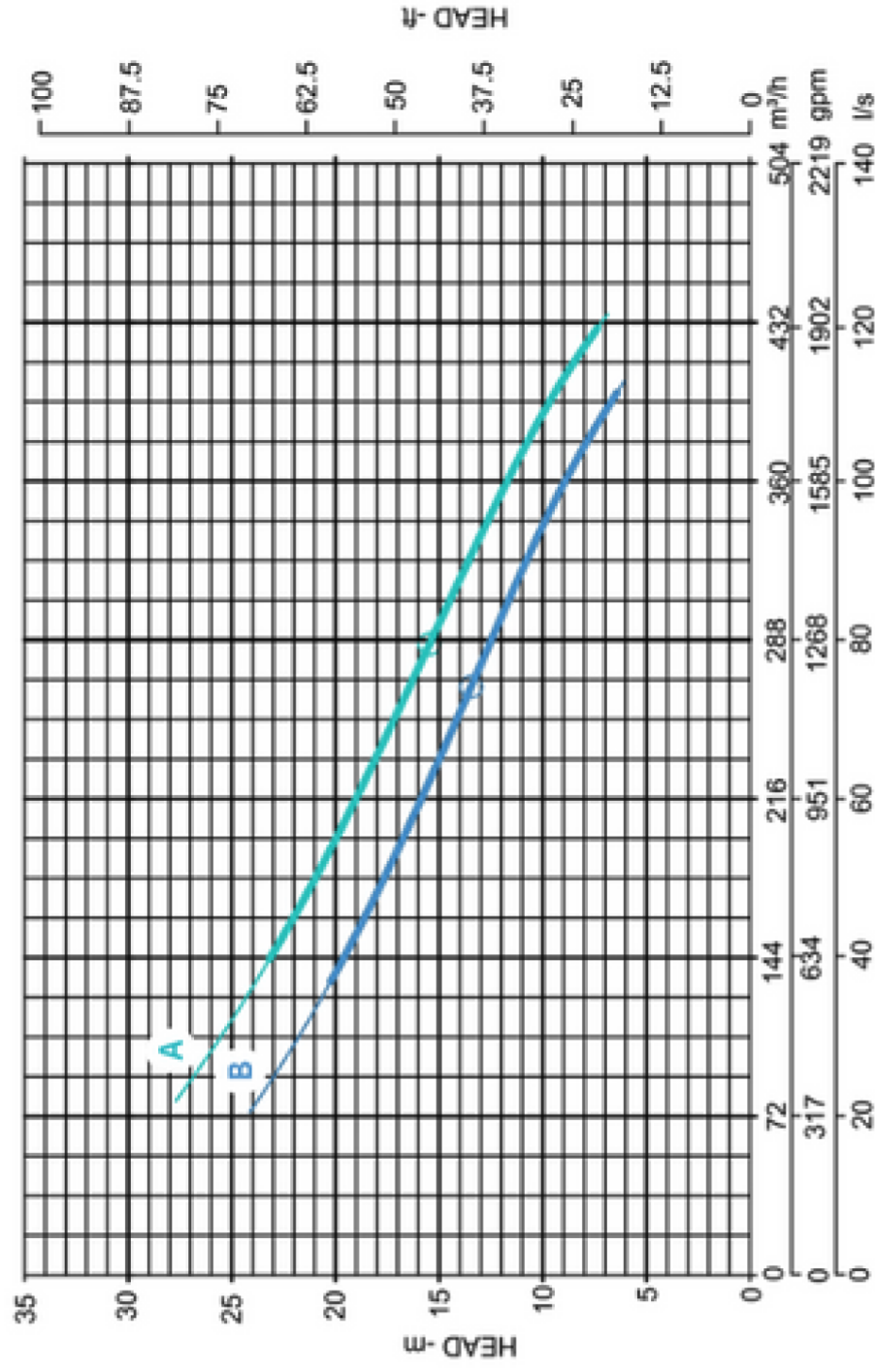
Curves at Speeds: A 1600 rpm B 1500 rpm
