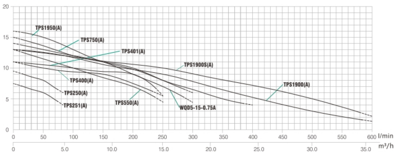
PERFORMANCE CHART AT n=2900rpm
