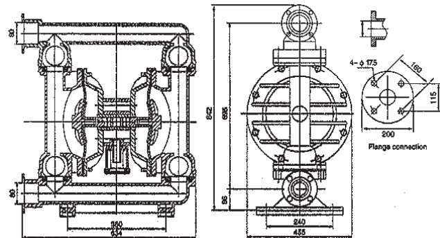
Installation Dimension
