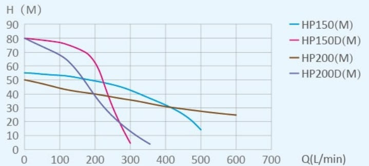
Performance Curve
