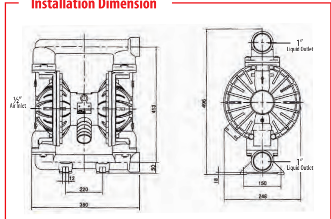
Installation Dimension
