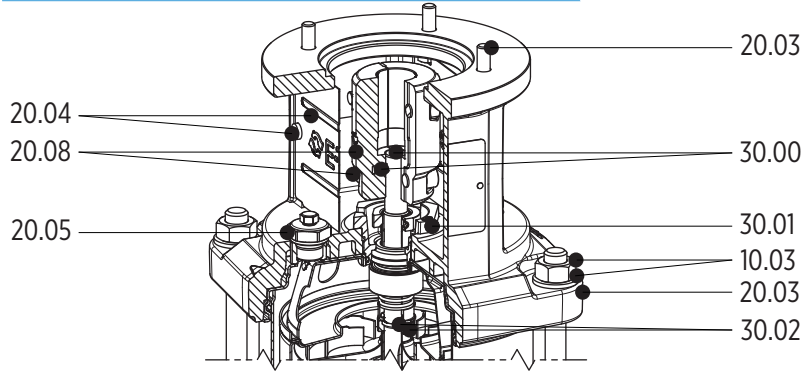
CONFIGURATION UP TO 4 KW WITHOUT THRUST BEARING
