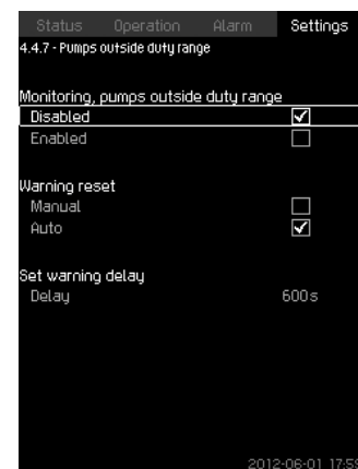
Fig. 33 Pumps outside duty range
