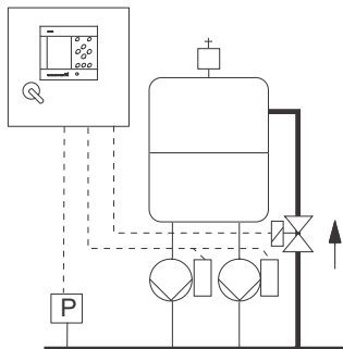
Fig. 36 Pressure-holding system
