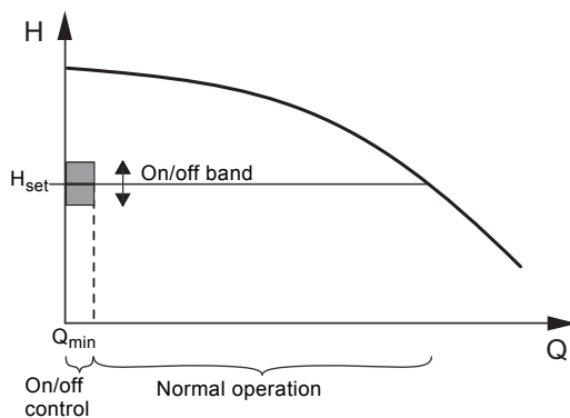
Fig. 23 On/off band
