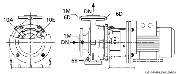
Double mechanical seal in back-to-back arrangement (DB)
