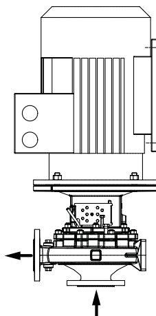
Pump sets, motor sizes 200 - 315, 2-pole
