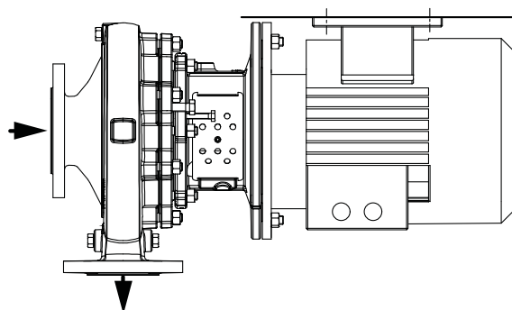
Pump sets, motor sizes 132 - 180
