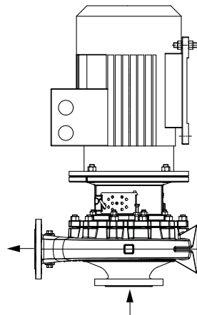
Pump sets, motor sizes 200 - 315, 4-pole
