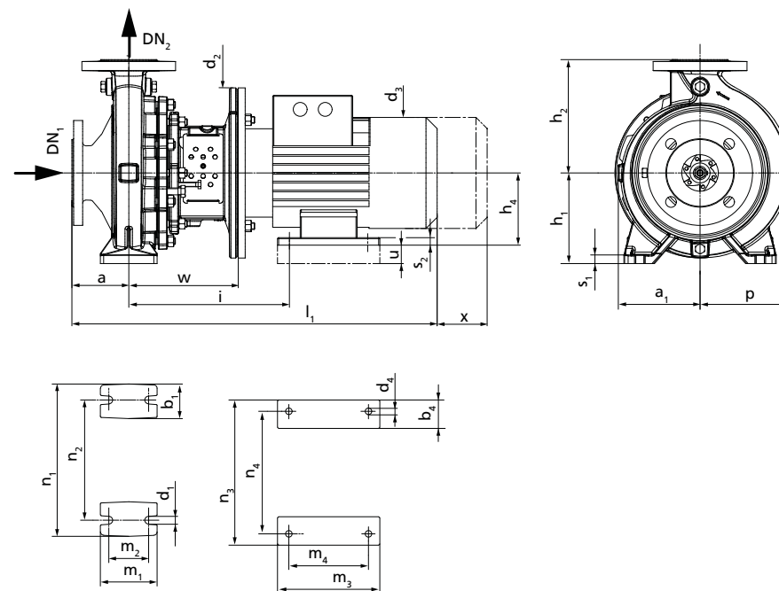
Pump set with volute casing foot and motor foot (motor sizes 132 to 180)
