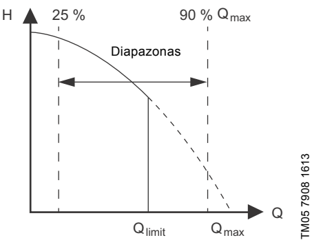
55. pav. FLOW LIMIT
