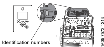
Fig. 2 Identification numbers
