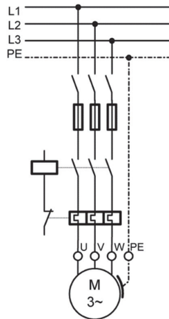
Figure 5-13: Direct starting
