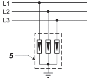
Figure 5-12: Surge voltage protection
