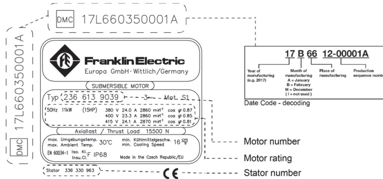
Figure 5-1: Type plate with date of manufacture
