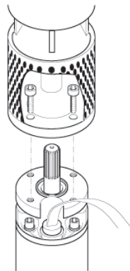
Figure 5-5: Pump assembly
