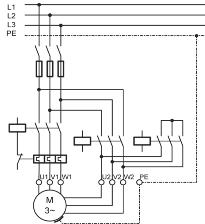
Figure 5-14: Wye-delta-starting
