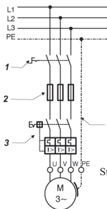
Figure 5-10: Fusing and motor protection
