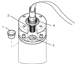
Figure 5-5: Connection of the short motor cable
