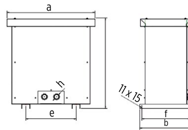
dV/dt filter connection plan
