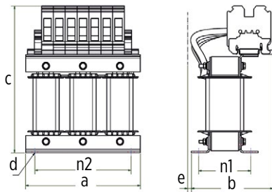
IP00 dV/dt filter outlines
