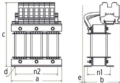
IP00 dV/dt filter outlines
