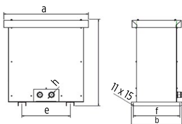
IP54 Sinus filter outlines floor mount
