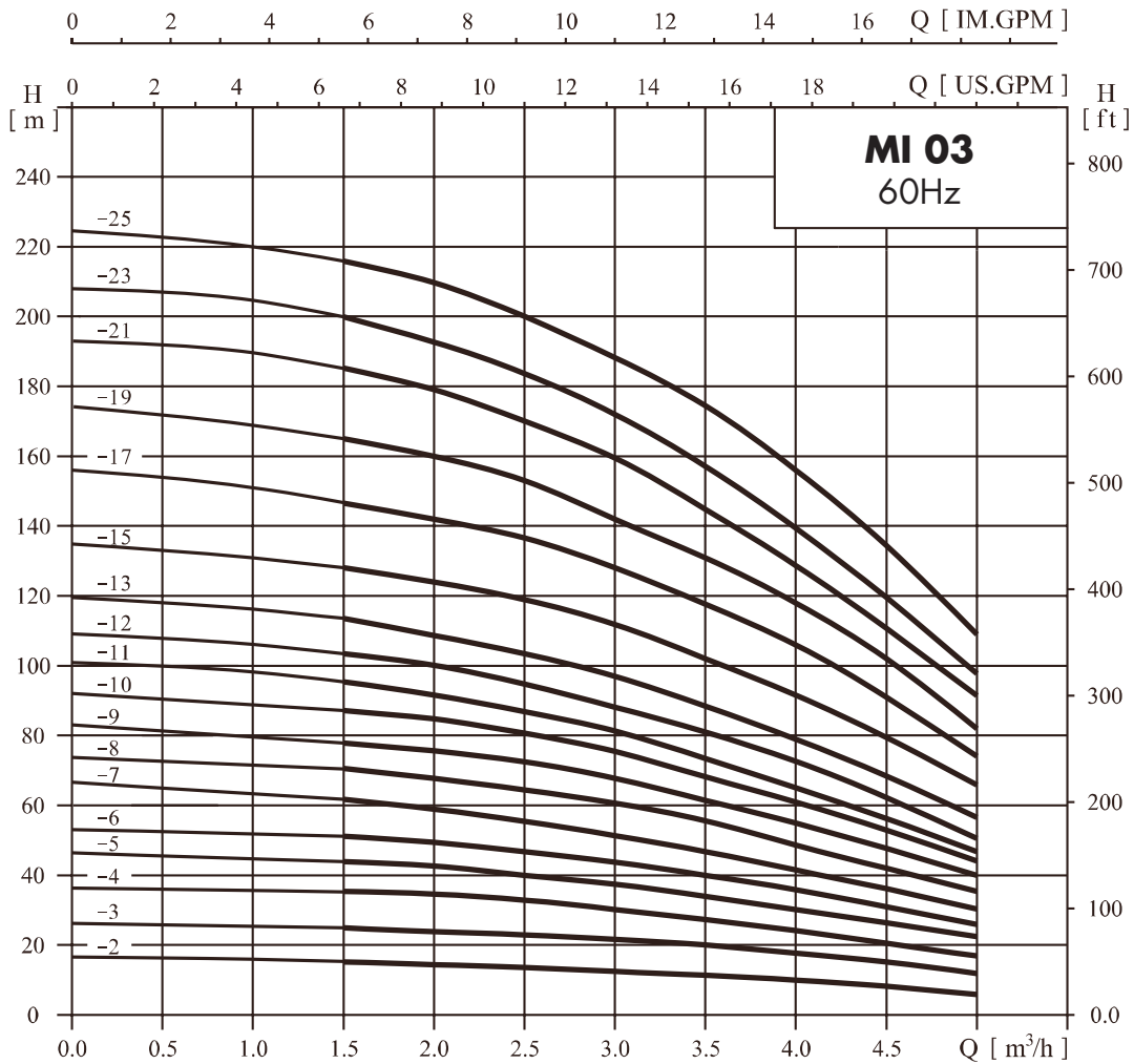
Performance curve ISO9906:2012 Grade 3B
