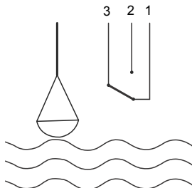
3. pav. To fill or alarm at low liquid level
