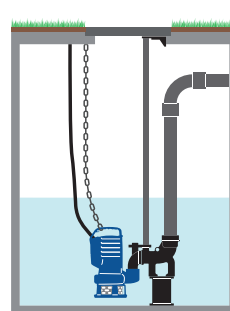
WITH BASE COUPLING FOOT [DAC-V - Page 79]
