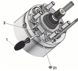
Figure 5-2: 6", 8", 10" motor
