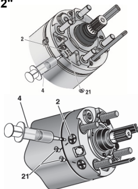
Figure 5-6: Topping up the motor fluid
