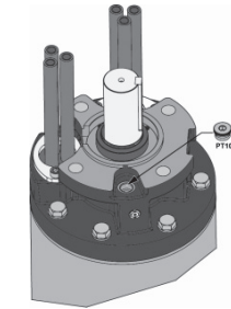
Figure 5-3: 12" motors
