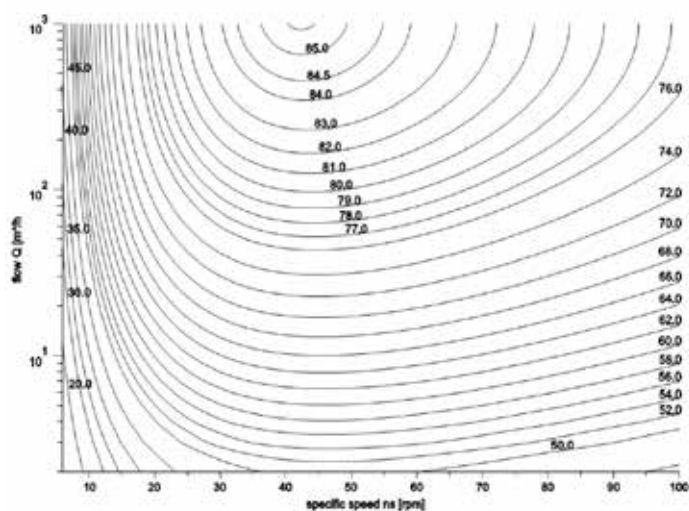
MEI = 0.4 for ESOB 1450
