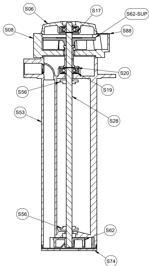
Spare parts nomenclature
